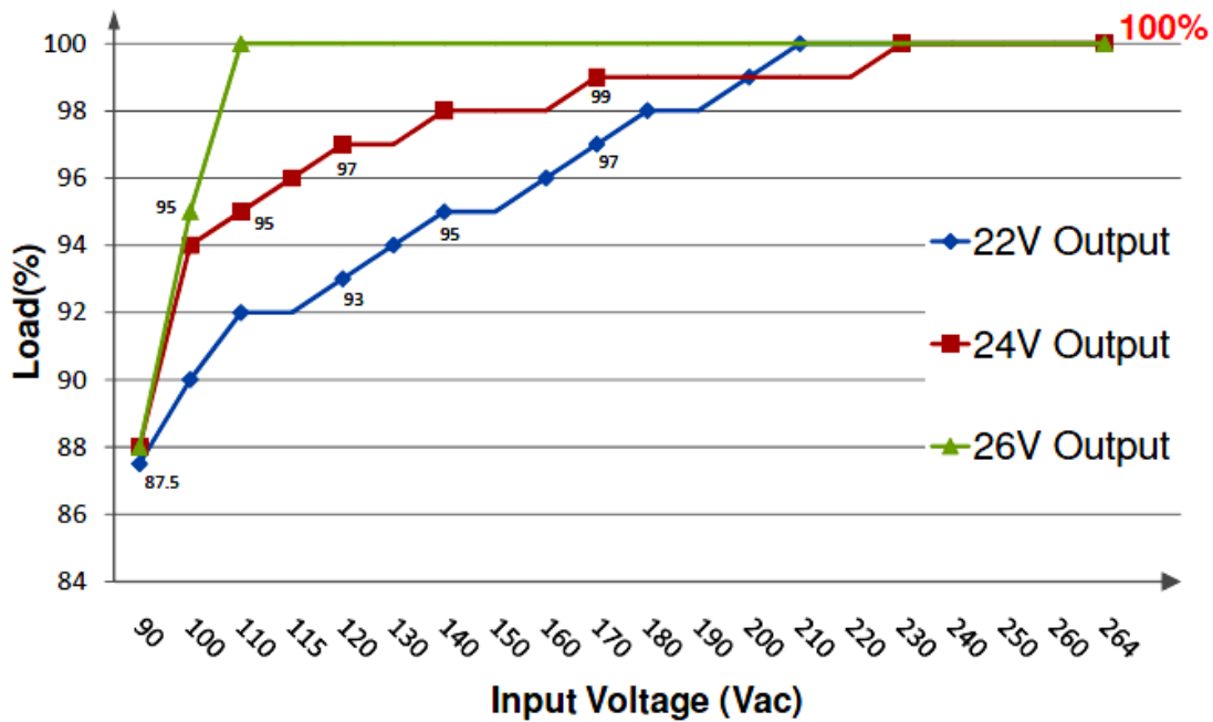
MPI-U405 with Convection Cooled @ ambient 50 degrees C
