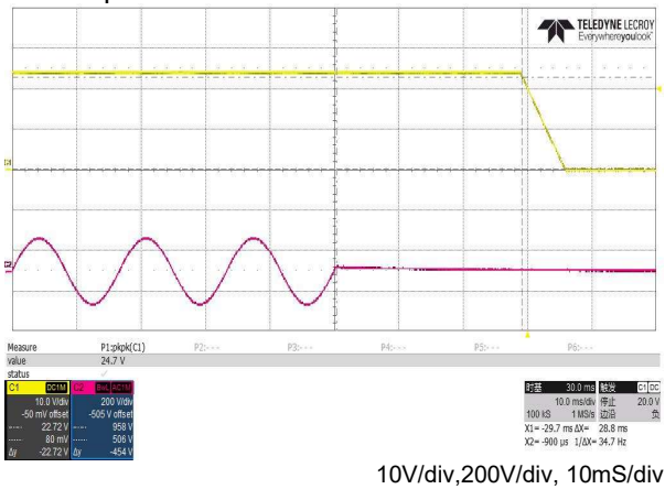
Hold-up time
