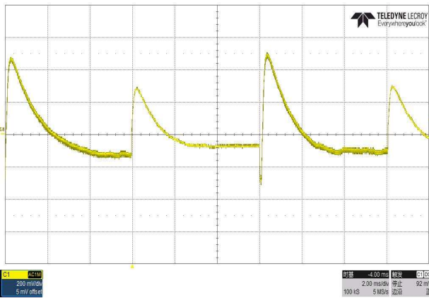
Step response
