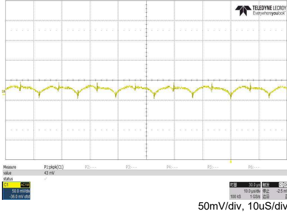
Switching frequency ripple
