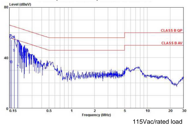
EMI: FCC "B" (Conduction)
