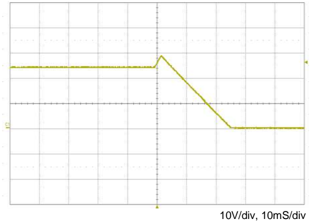
OVP 60% of rated load
