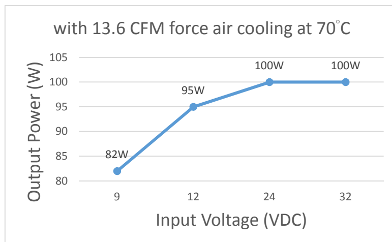
Performance curves (with fan) at 70°C
