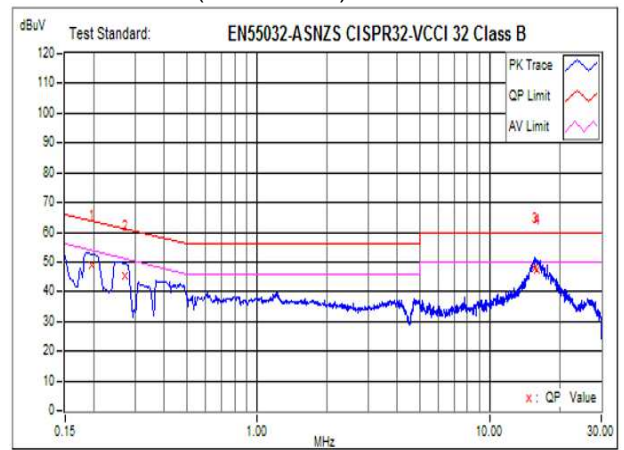
EMI: FCC "B" (Conduction)
