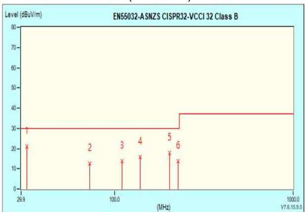
EMI: EN 55032 "B" (Radiation)
