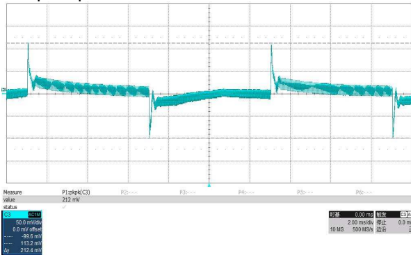
Step response 20%~100% of rated load
