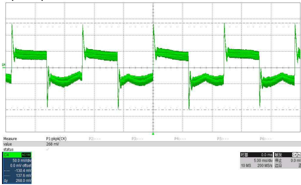
50mV/div, 5mS/div
