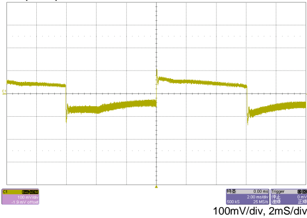
Step response 20%~100% of rated load
