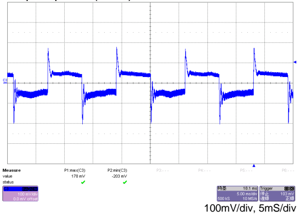
Step response (115V) 20%~100% of rated load
