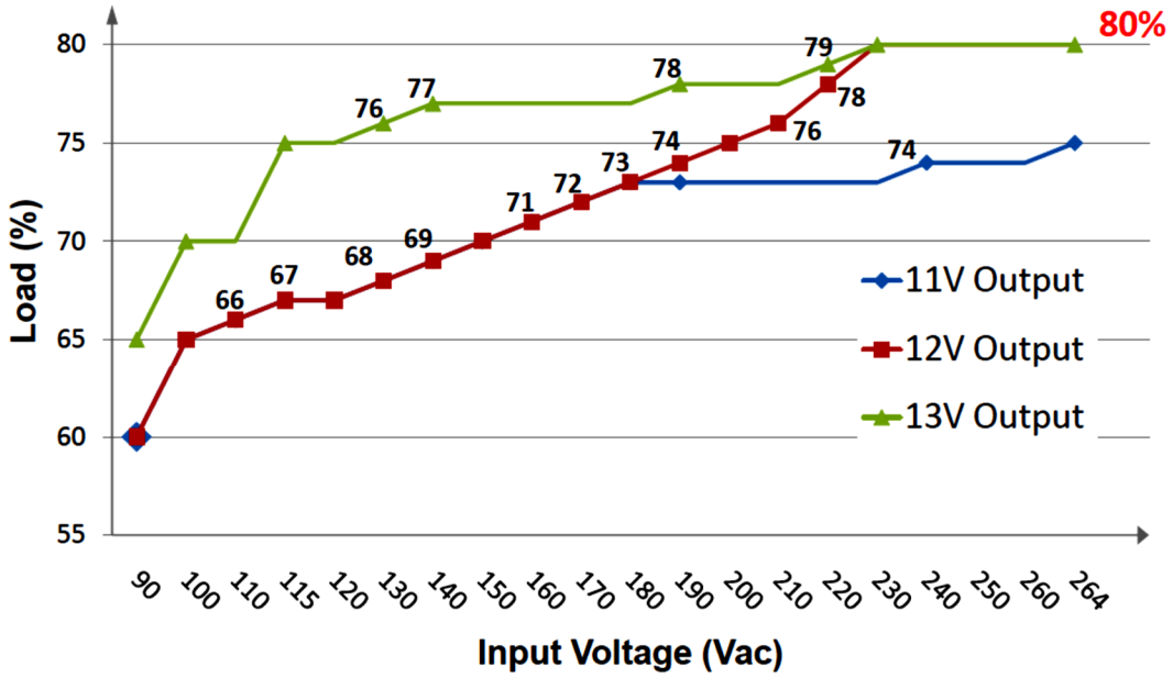
MPI-U403 with Convection Cooled @ ambient 70 degree C
