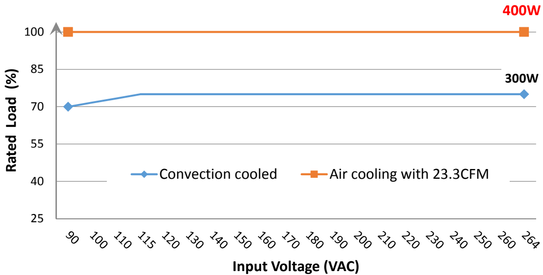
Performance curves of MPI-U403-C (12V output @ 50°C)
