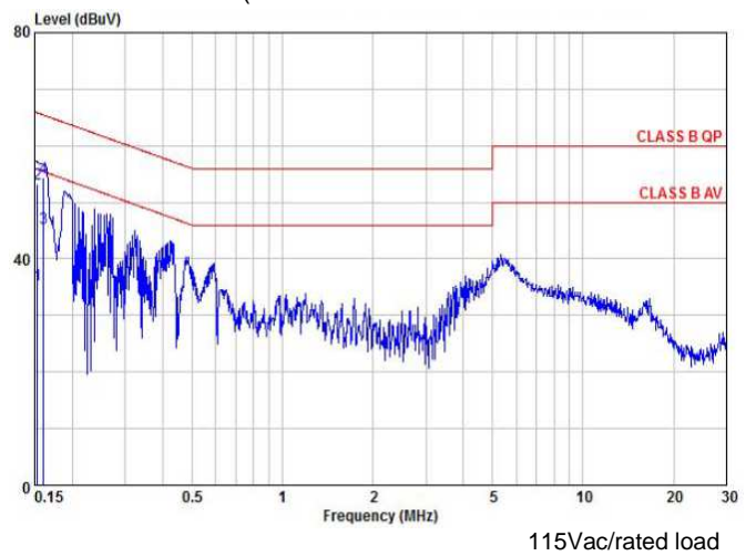
EMI: FCC "B" (Conduction)
