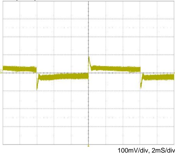
Step response 20%~100% of rated load
