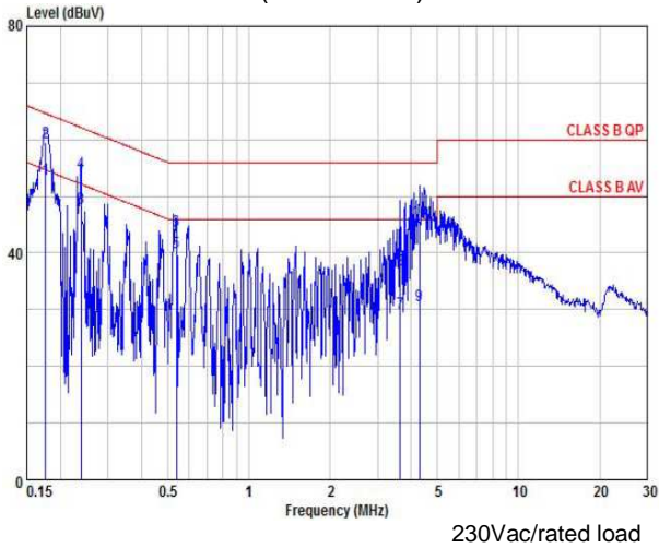
EMI: EN55011 "B" (Conduction)
