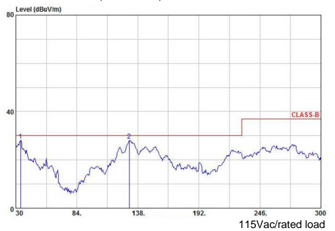
EMI: FCC "B" (Radiation)
