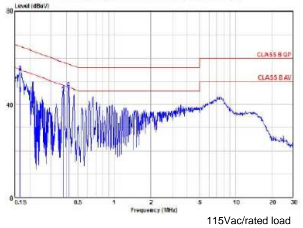
EMI: FCC "B" (Conduction)
