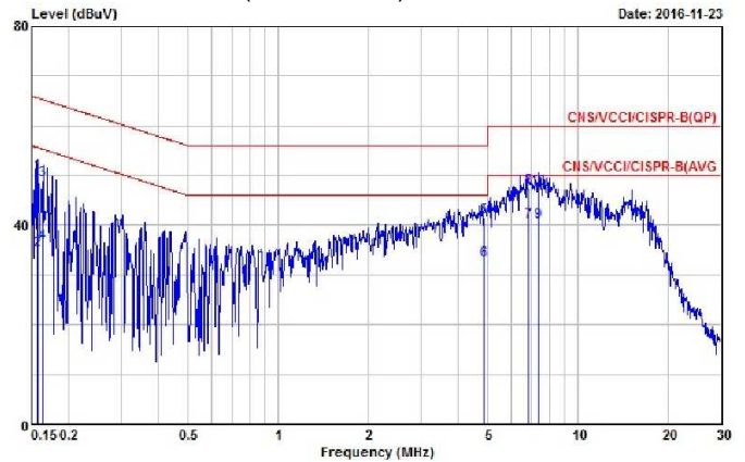
115Vac/rated load
