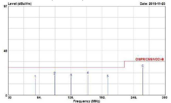
115Vac/rated load
